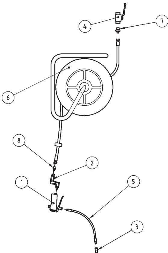
Slangupprullare, 10 m, med matarventil Art.nr: 200098 Hose reel, 10 m, with grease gun Art.No: 200098
