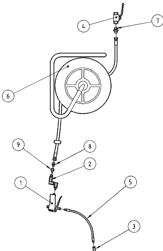
Slangupprullare, 15 m, med matarventil Art.nr: 200099 Hose reel, 15 m, with grease gun Art.No: 200099
